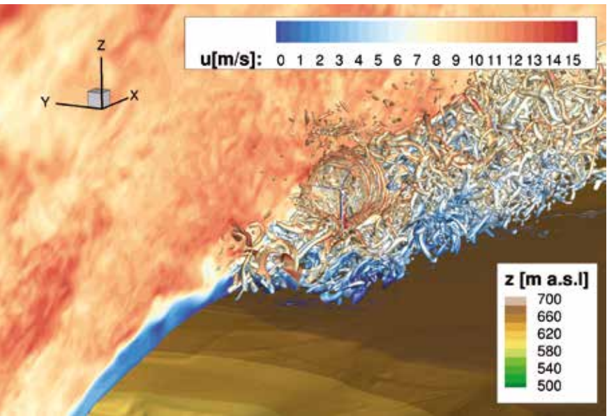
Uni Stuttgart researchers are running ultra-high-resolution detached eddy simulations as part of the WINSENT project. This image shows the topography on the ground, color coded by elevation. Above, a vertical plane depicts the flow fields, colored by the value of the horizontal wind velocity. There are also turbulent structures highlighted in the flat plateau on top of the hills, also colored to represent wind speed. © Patrick Letzgus, Uni Stuttgart
